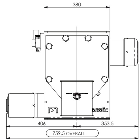
WITH FORCED VENTILATION FOR SCREW FEEDER ENGINE
