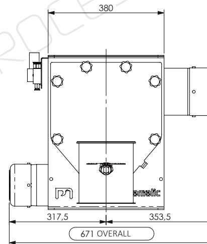
WITHOUT FORCED VENTILATION FOR SCREW FEEDER ENGINE
